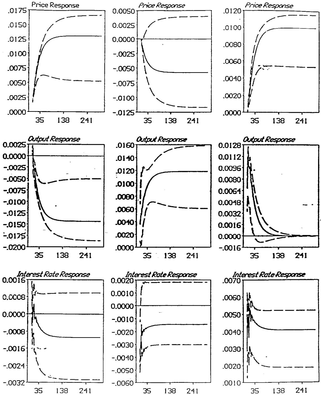
Figure 3: Responses of Total IP, CPI All Items and the Fed Funds Rate to \epsilon Shocks to \delta Shocks to \omega Shocks
