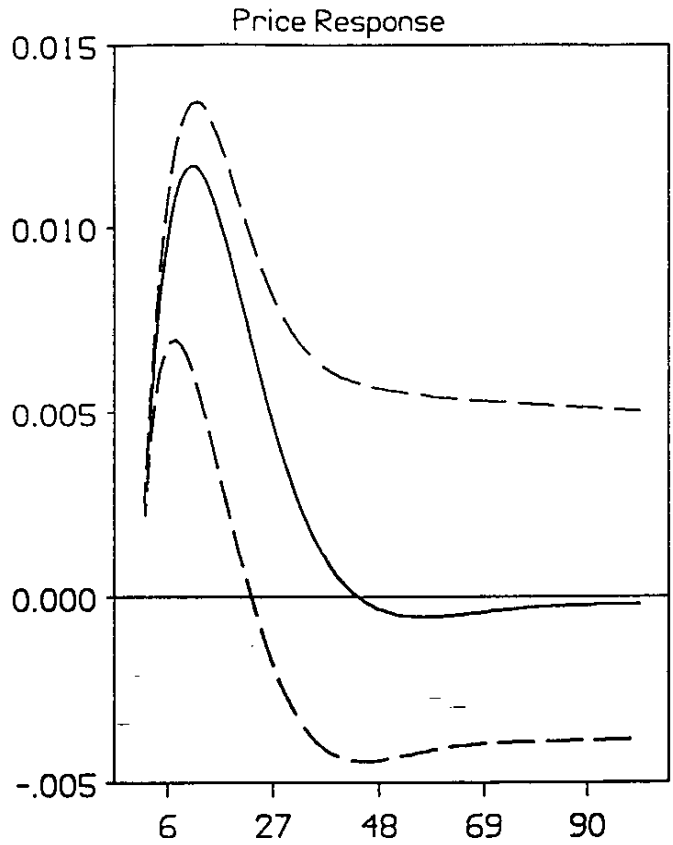
Figure 1: Responses of GDP and the GDP Deflator to \epsilon Shocks to \gamma Shocks
