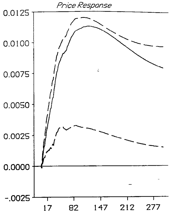
Figure 2: Responses of Total IP and CPI All Items to \epsilon Shocks to \epsilon Shocks to \gamma Shocks
