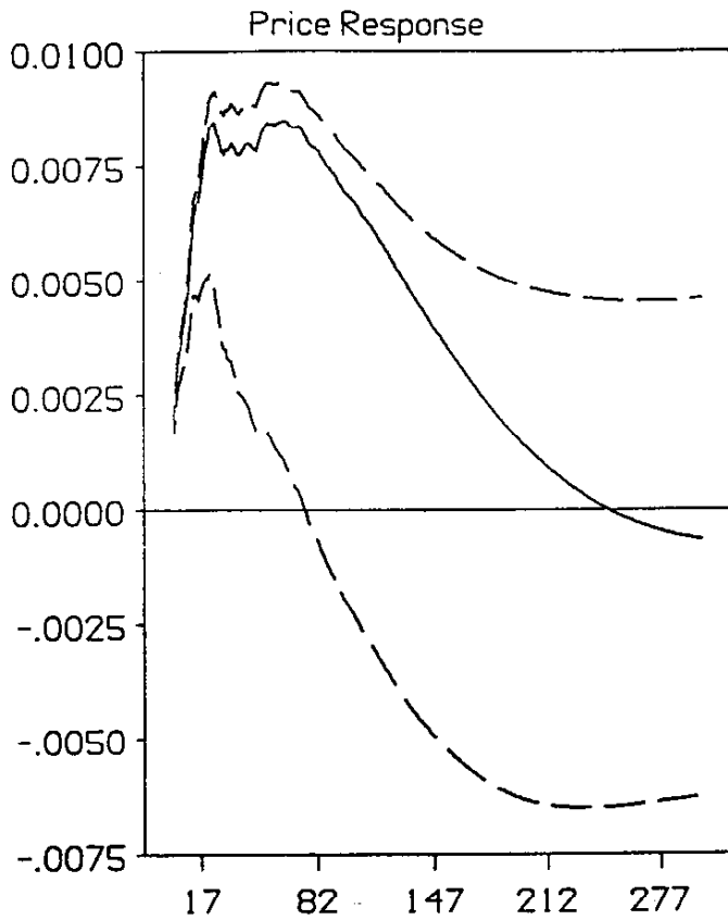
Figure 2: Responses of Total IP and CPI All Items to \epsilon Shocks to \epsilon Shocks to \gamma Shocks
