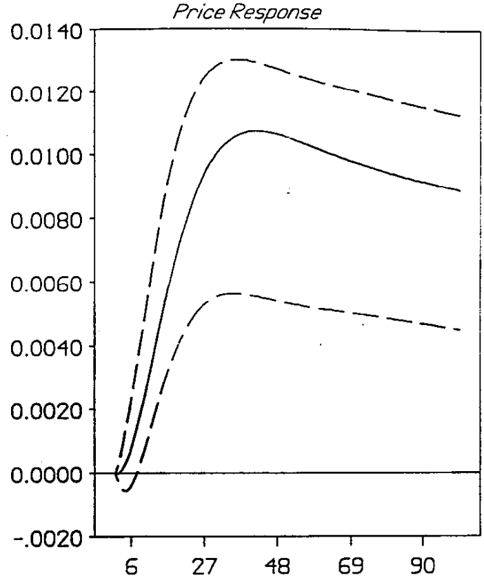
Figure 1: Responses of GDP and the GDP Deflator to \epsilon Shocks to \gamma Shocks
